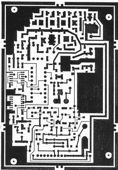
PLL UNIT SOLDER FOIL SIDE FOR THE AR2002 SERIAL NUMBERS 1500 UP
